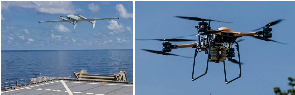
Near Earth's Firefly Compact Autonomy System on L3 Harris FVR-90 (Left) and BAE TRV-150 (Right)
